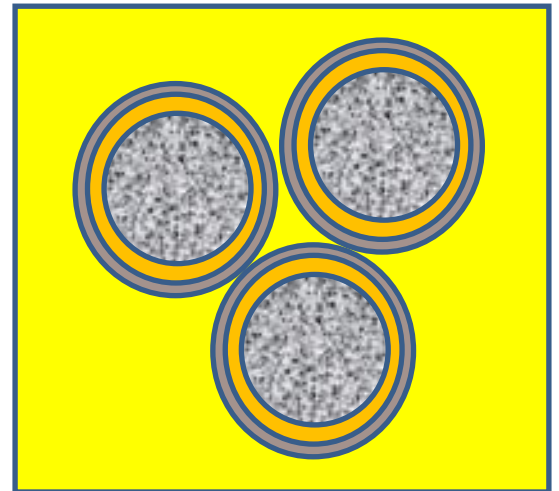
Triangular unit cell for placing fuel elements, pitch 17.6 mm.
