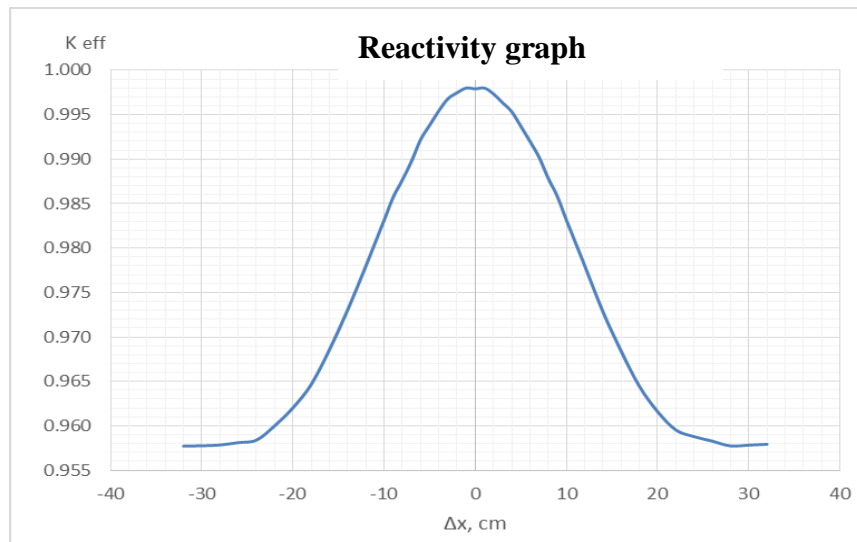
Graph of the modulator reactivity; in the region of \pm 5 \text{ cm} from the maximum the reactivity is described by a parabola with a parameter 10^{-4} k_{eff}/\text{cm}^2 .
